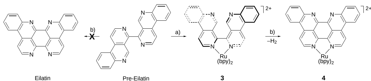
Scheme 3. Dehydrogenation of [Ru(bpy)_2(\text{pre-eilatin})]^{2+} ( 3 ) to [Ru(bpy)_2(\text{eilatin})]^{2+} ( 4 ). Reagents and conditions: a) [Ru(bpy)_2Cl_2] \cdot 5H_2O , ethylene glycol–water 1:1, 100 °C, 3 h, 62 % yield; b) Pd/C, ethylene glycol–acetone 10:1, 175–190 °C, 1 h, 97 % yield. All complexes were isolated as their PF_6^- salts. [10] Note that identical reaction conditions do not convert the free pre-eilatin ligand to eilatin.
