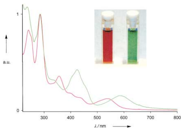
Figure 2. UV/Vis spectra of 3 (red) and 4 (green) in CH_3CN . Inset: a picture of the corresponding solutions.
