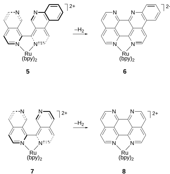
Scheme 4. Dehydrogenation reactions of 5 and 7 to yield the novel complexes 6 and 8 , respectively. All complexes were isolated as their PF_6^- salts. [10]
